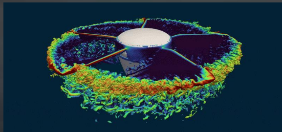
Unducted Rotor
